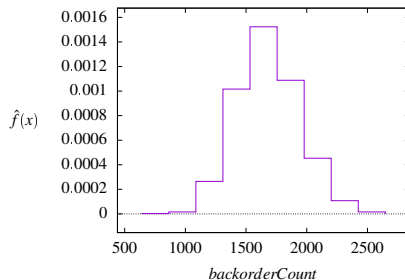
backorderCount Density Histogram
