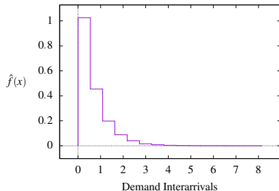
Exponential(2/3) Density Histogram
