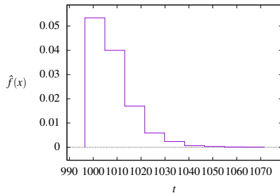
t Density Histogram
