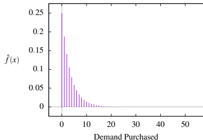
Exponential(7) Density Histogram
